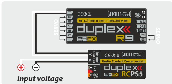
Fig. 5: Application connection with RC Power Switch
