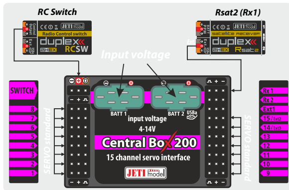
Fig. 4: Application connection with RC Switch
